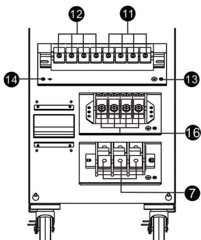
Diagram 3: Ranger 60KT, terminal intrare/iesire
