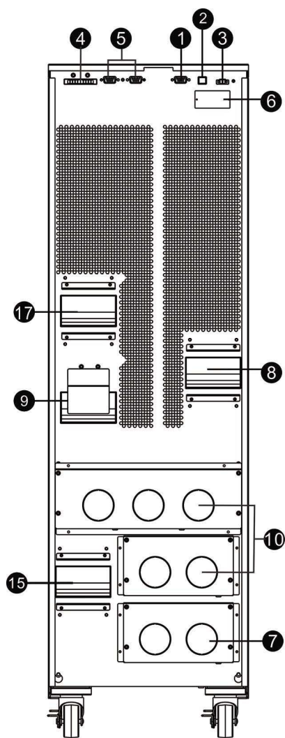
Diagram 2: Ranger 60KT panou spate
