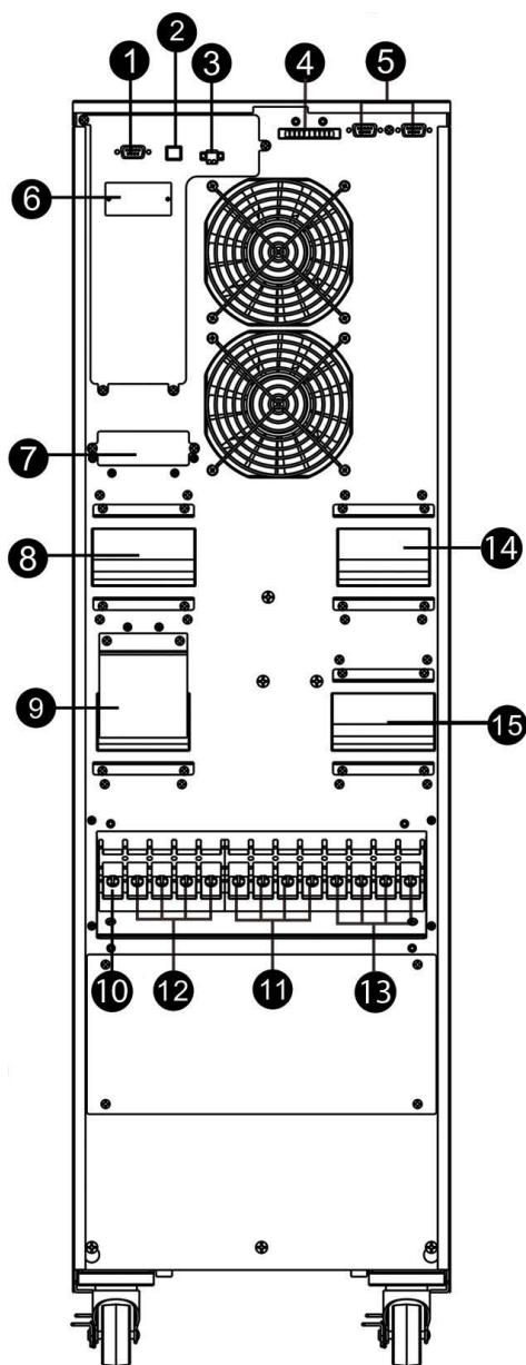
Diagrama 1: Ranger 30KT Panou spate
